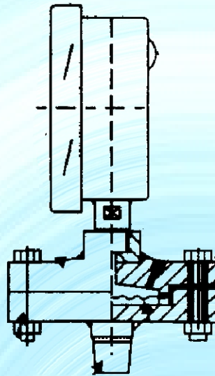
Bottom Entry Direct Mounting
