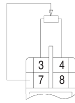
3-wire compensation for transfer resistance {4}
