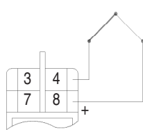
Internal CJC-compensation
