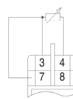
3-wire cable compensation
