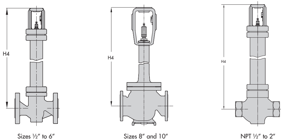
Type 3241 (241) Globe Valve with insulating section or metal bellows seal
