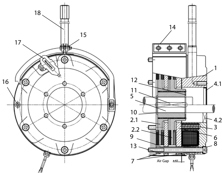
Figure 2: Brake models ZS(X)300A, ZS(X)500A.
