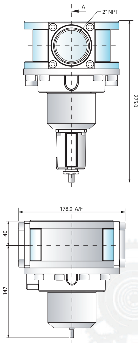
Filter with manual drain
