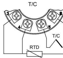
External CJC-compensation 3-wire cable compensation
