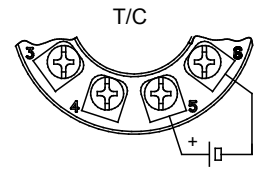
Voltage measurement
