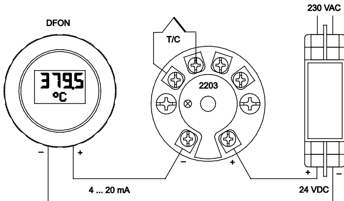
External CJC-compensation No cable compensation Can be configured
