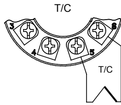
Internal CJC-compensation
