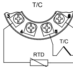
External CJC-compensation No cable compensation Can be configured
