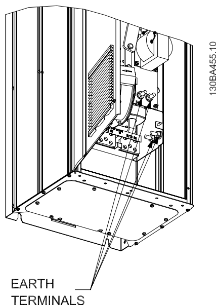
EARTH TERMINALS Figure 3.43: Position of ground terminals IP21 (NEMA type 1) and IP54 (NEMA type 12)
