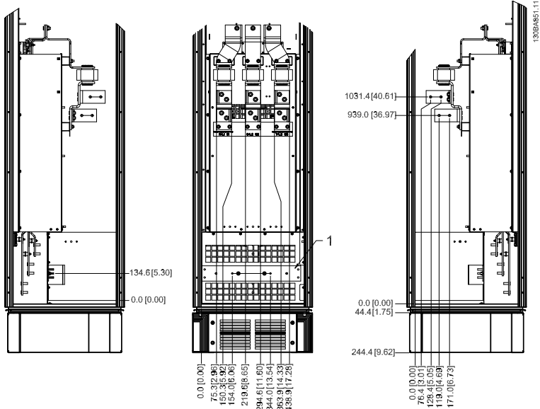
Figure 3.25: Terminal locations - Options cabinet (left side, front and right side view). The connector plate is 1.65 in [42 mm] below .0 level. 1) Earth ground bar
