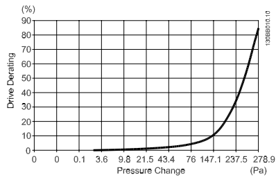
Figure 3.28: E frame Derating vs. Pressure Change (Small Fan), P250T5 and P355T7-P400T7 Drive airflow: 650 cfm (1105 m³/h)
