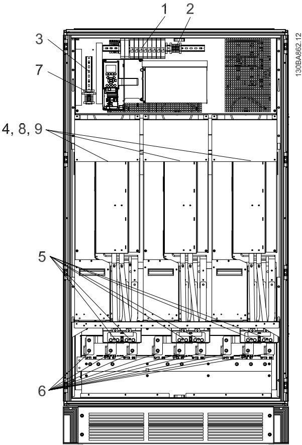
Figure 3.49: Inverter Cabinet, frame size F2 and F4
