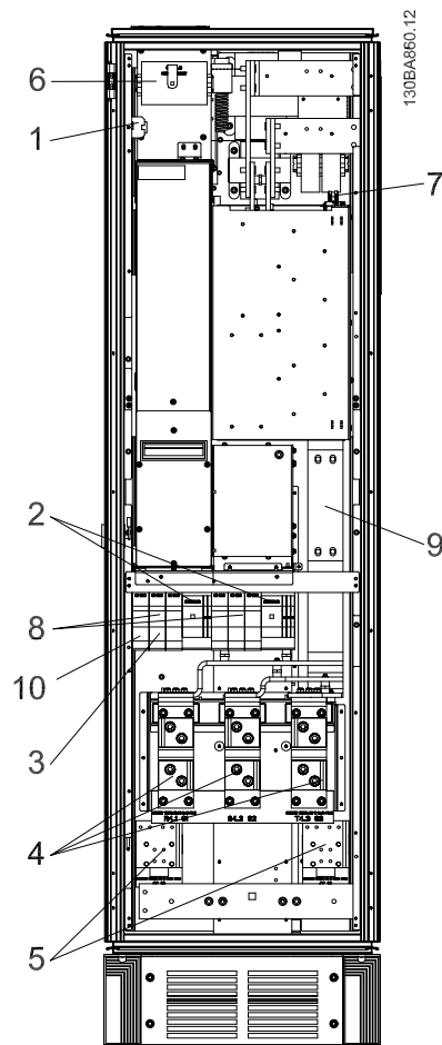
Figure 3.47: Rectifier Cabinet, frame size F1, F2, F3 and F4
