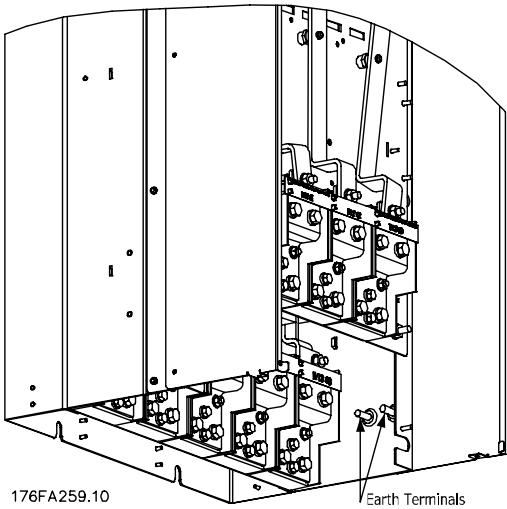
Figure 3.46: Position of ground terminals IP00, frame sizes E
