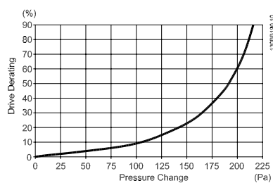
Figure 3.30: F1, F2, F3, F4 frame Derating vs. Pressure Change
