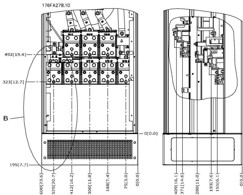
Figure 3.15: IP21 (NEMA Type 1) and IP54 (NEMA Type 12) enclosure power connection positions
