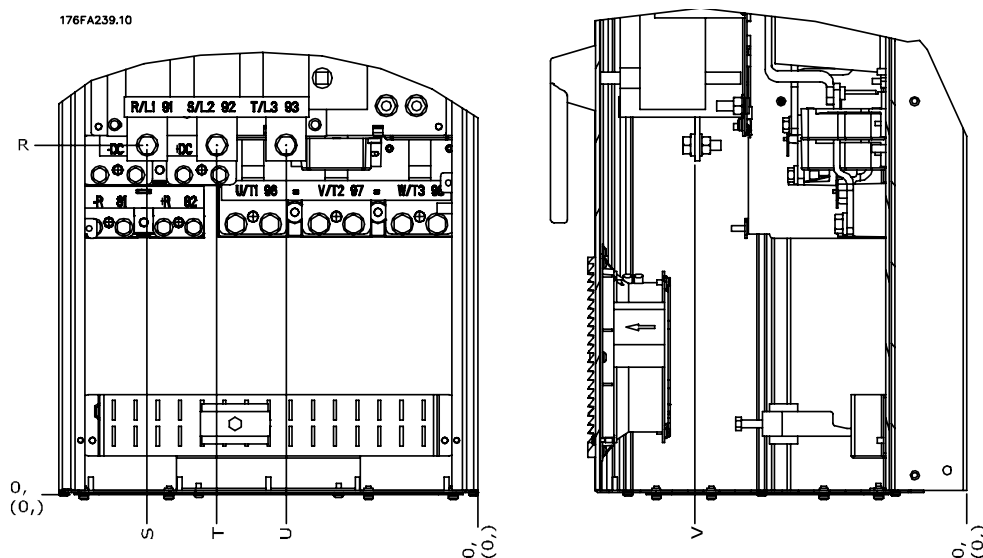
Figure 3.14: Position of power connections with disconnect switch, frame size D1 and D2
