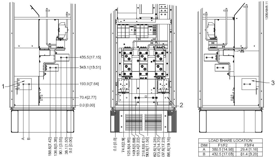
Figure 3.24: Terminal locations - Rectifier (left side, front and right side view). The connector plate is 1.65 in [42 mm] below .0 level. 1) Load Share Terminal (-) 2) Earth ground bar 3) Load Share Terminal (+)
