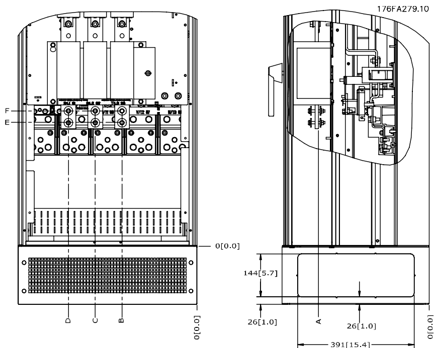
Figure 3.17: IP21 (NEMA type 1) and IP54 (NEMA type 12) enclosure power connection position of disconnect switch
