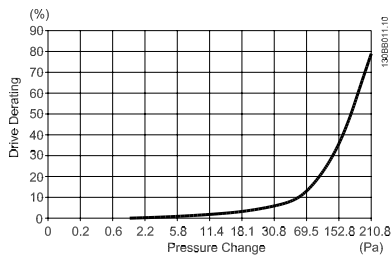
Figure 3.29: E frame Derating vs. Pressure Change (Large Fan), P315T5-P400T5 and P500T7-P560T7 Drive airflow: 850 cfm (1445 m³/h)
