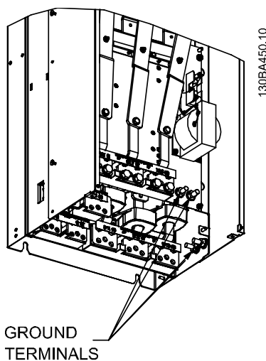
GROUND TERMINALS Figure 3.42: Position of ground terminals IP00, frame sizes D
