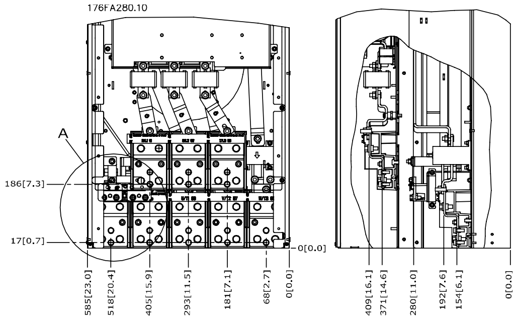
Figure 3.18: IP00 enclosure power connection positions
