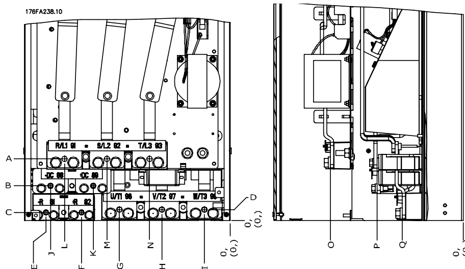
Figure 3.13: Position of power connections, frame size D3 and D4
