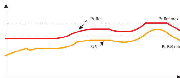
Floating condensing temperature set point control by VLT® Refrigeration Drive FC 103.
