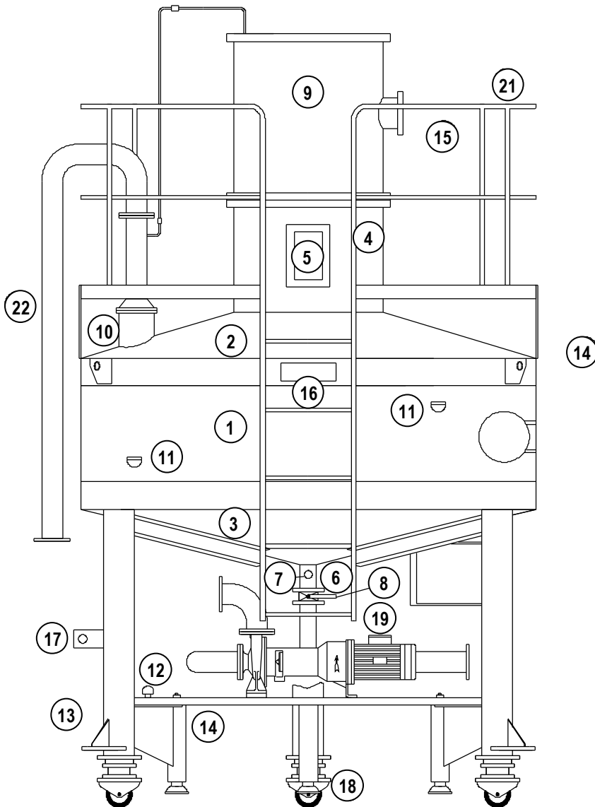
Typical drawing of 5.000 litres Tank prover with different options
